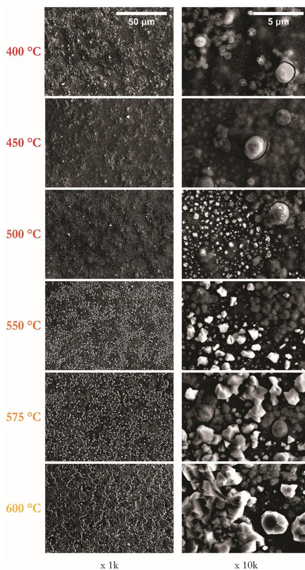
Fig. 3 Series of representative SEM images of CZTS thin films as a function of annealing temperature from 400 to 600 °C at 1 hour shown at magnifications of 1k and 10k.
