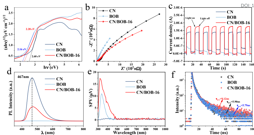
Fig. 6 (a) (ah\nu)^{1/2} - h\nu UV-Vis DRS spectra; (b) EIS measurement results; (c) Transient photocurrent response; (d) Photoluminescence spectra; (e) SPV spectrum; (f) PL decay curves of g-C 3 N 4 /Bi 4 O 5 Br 2 -16 and g-C 3 N 4 .
