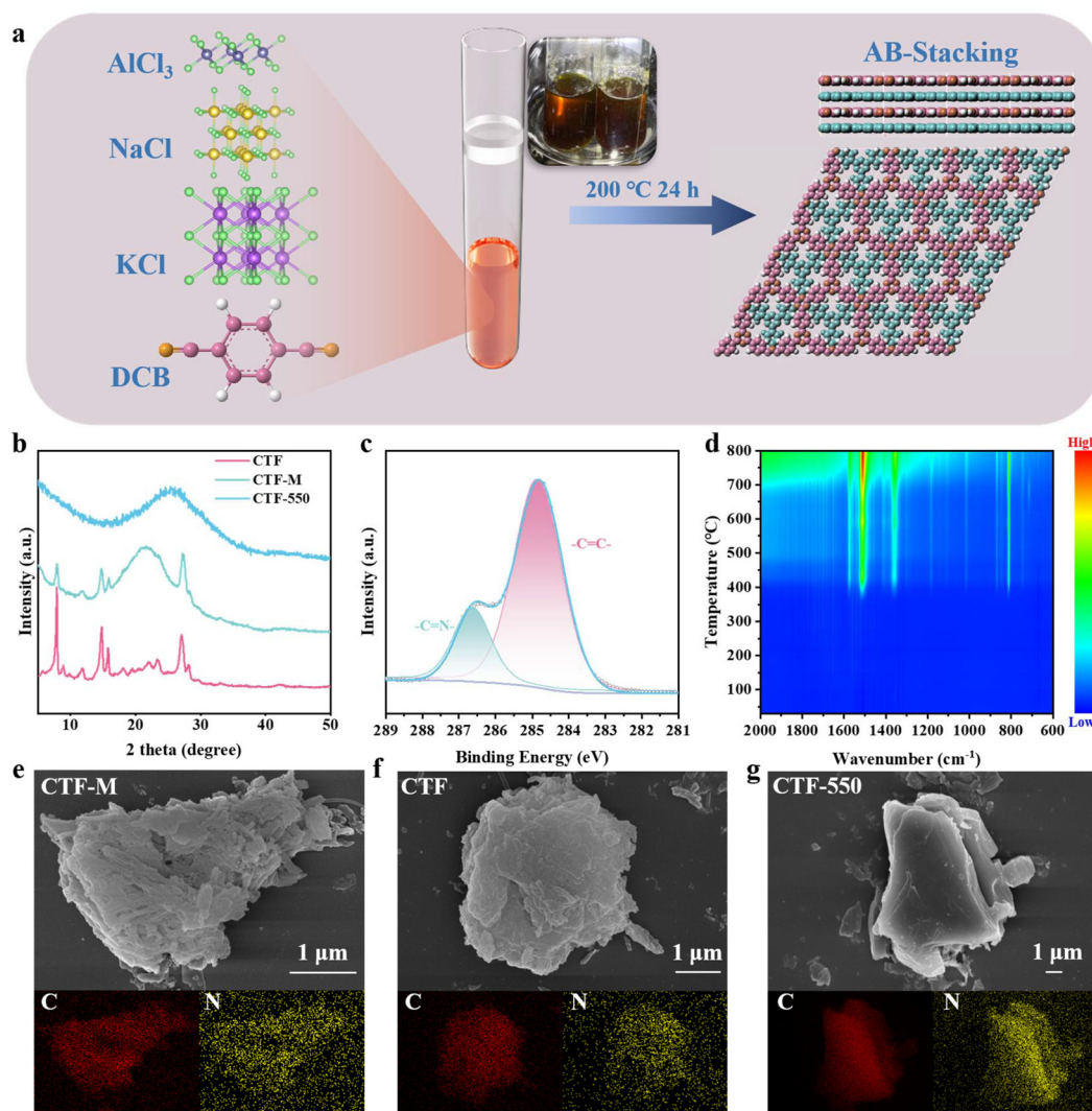
Fig. 1 (a) Illustration of the preparation process of CTFs. (b) The XRD patterns of CTF, CTF-M and CTF-550. (c) The \text{C } 1\text{s} XPS spectra of CTF. (d) The TG-FTIR spectra of CTF. The SEM images and C and N elemental mapping images of (e) CTF-M, (f) CTF, (g) CTF-550.
