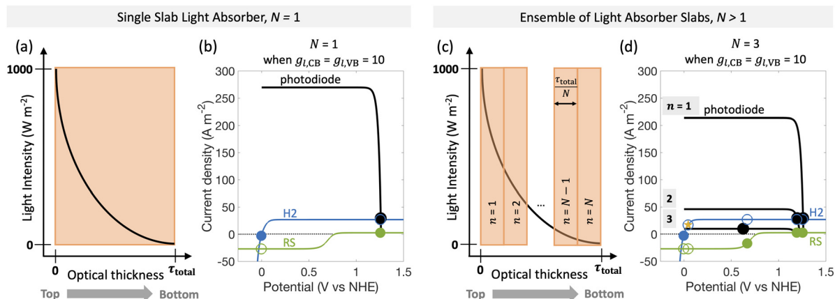
Fig. 6 Qualitative incident light intensity profiles for (a) a single light absorber slab, N = 1 , and (c) for an ensemble of light absorbers, N > 1 , where space between the slabs has been omitted because it is assumed to be optically transparent. In both cases, the incident light exponentially decreases in intensity (y-axis) with increasing depth from the top to the bottom of the reactor (x-axis); n \in [1, N] represents the spatial position of the different light absorbers moving from the top ( n = 1 ) to the bottom ( n = N ). (b) and (d) Load-line analysis depicting a photodiode power curve (black), individual reaction load curves (H 2 : hydrogen reaction in blue, RS: redox shuttle reaction in green) for (b) N = 1 and (d) N > 1 . Current densities for the desired redox reactions of H 2 evolution and RS oxidation are shown by the filled markers, the competing reactions are shown by the open markers, and the overall operating point of the device is indicated by black markers. Star marker indicates shift towards H 2 oxidation at CB for n = 3 .
