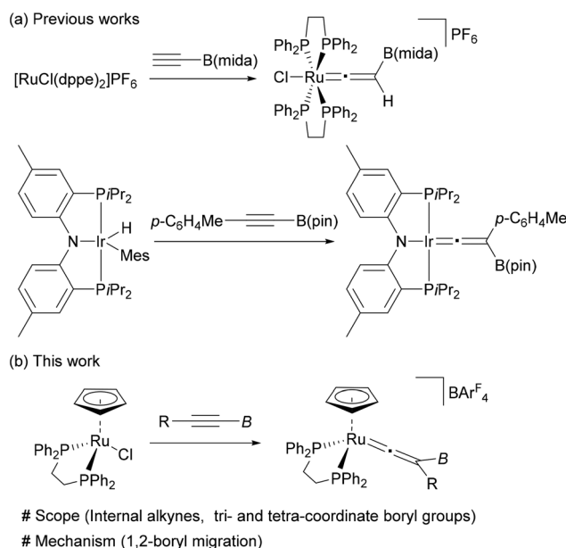
Fig. 1 Vinyldiene rearrangements of borylalkynes.
