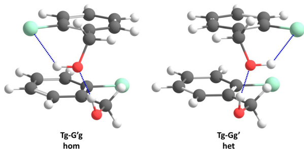
Fig. 2 Comparison of the most stable homochiral (ochiral) with the most stable het(erochiral) Cl dimer structure. The enantiomeric acceptor units lead to a large difference in the Cl-Cl atom distance.
