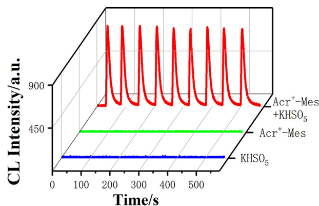
Fig. 7 CL intensity-time curves of \text{KHSO}_5 , \text{Acr}^+\text{-Mes} , and \text{Acr}^+\text{-Mes/KHSO}_5 systems. [ \text{Acr}^+\text{-Mes} ]: 0.1 \text{ mM} ; [ \text{KHSO}_5 ]: 2 \text{ mM} ; [PBS]: 0.1 \text{ M} , pH = 7; PMT voltage: -900 V. Reprinted with permission from ref. 15, Copyright 2023 American Chemical Society.
