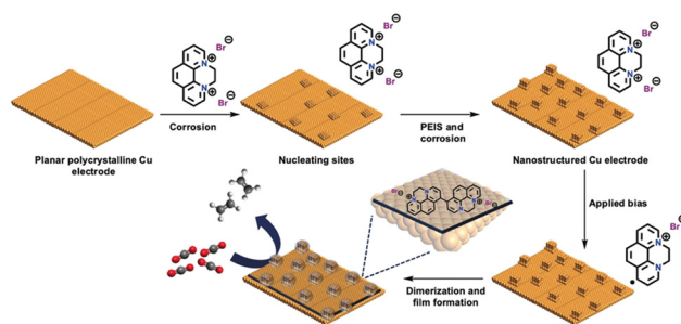
Fig. 14 Pictorial representation of the model for nanostructuring of a polycrystalline copper electrode and film electrodeposition by dimerization of N,N'-ethylene-phenanthroline dibromide. The combination of film and nanostructuring leads to high C_{\geq 2} selectivity for CO_2RR electrocatalysis. Reproduced with permission from ref. 86. Copyright 2019 Wiley.
