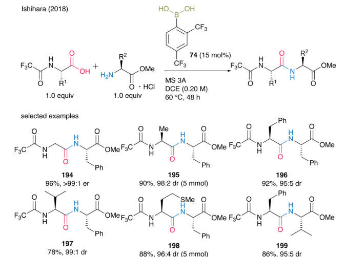
Scheme 42 2,4-Bis(trifluoromethyl)phenylboronic acid-catalyzed peptide bond formation reported by Ishihara. 28
