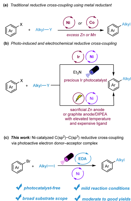
Scheme 1 Currently available C(sp 2 )-C(sp 3 ) reductive cross-coupling processes and the newly developed method via EDA complex.
