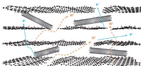
Fig. 3 Proposed mixed proton and electron conducting pathway of GO/Ox-SWCNT.
