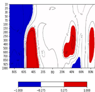
Fig. 8 Latitude–altitude section for slopes of September and October Antarctic oscillation index (SO–AAOI) and mean zonal (80 °E–130 °E) geopotential height. The abscissa represents latitude, while the ordinate represents pressure levels. The marked area passed the significance test at a 90% confidence level.
