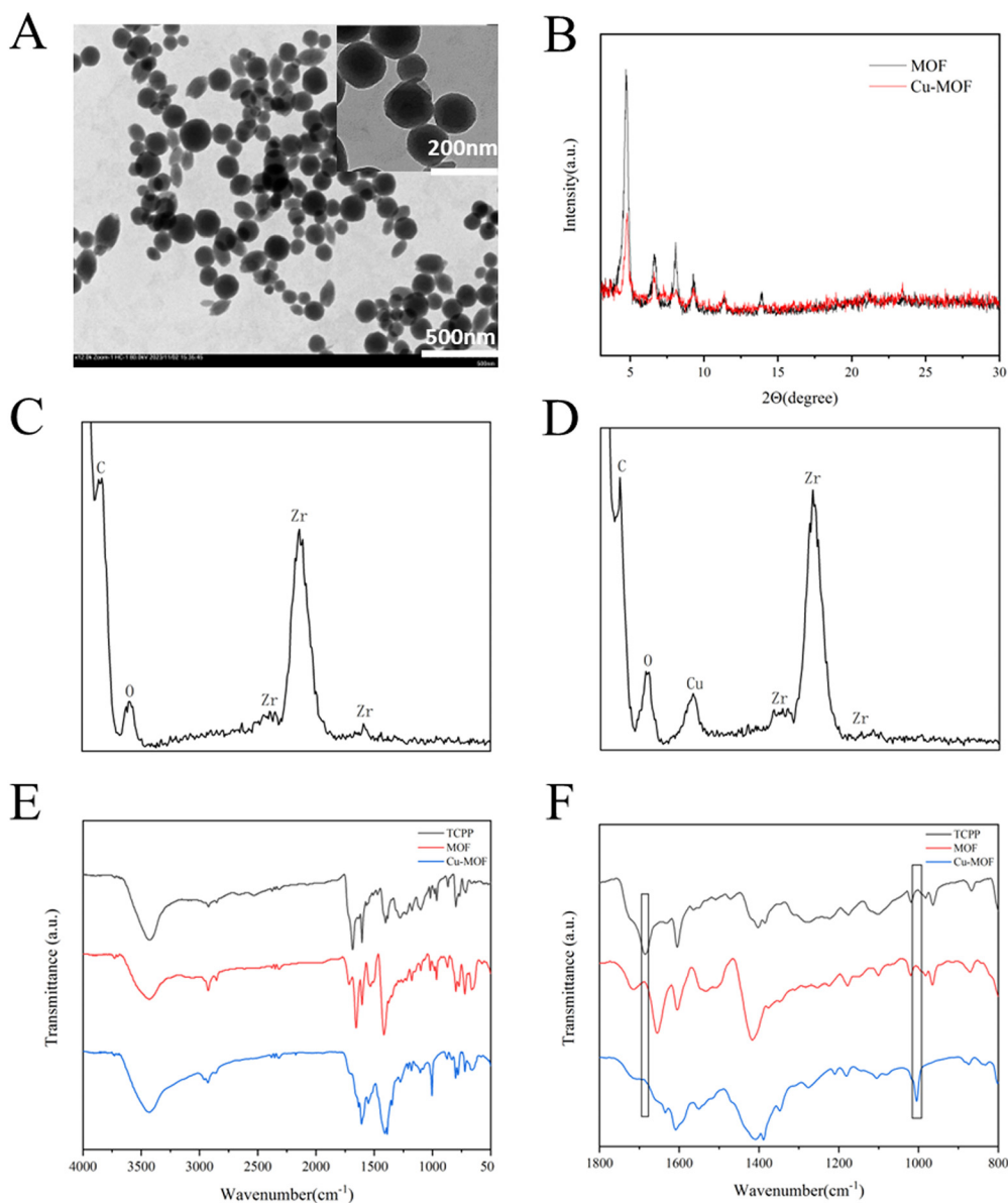
Fig. 1 (A) The TEM images of Cu-MOFs. (B) The XRD patterns of MOFs and the Cu-MOF. (C) The EDS analysis of the element composition of MOFs. (D) The EDS analysis of the element composition of the Cu-MOF. (E) The FTIR spectra of TCPP, MOFs and Cu-MOFs. (F) The magnified FTIR spectra of TCPP, MOFs and Cu-MOFs.
