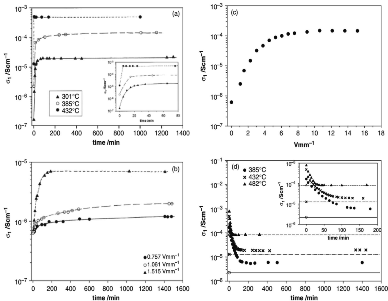
Fig. 2 Bulk conductivity of \text{BaTi}_{0.99}\text{O}_{2.98} (a) at different temperatures and times with a voltage of 10 V and field 15.1 \text{V mm}^{-1} , (b) at different voltages and times at 335 °C, (c) limiting conductivity for different voltages at 335 °C and (d) recovery at different temperatures on removal of the bias voltage (horizontal lines indicate the initial conductivity before voltage application); reproduced from H. Beltran et al. , J. Am. Ceram. Soc. , 2011, 94, 2951 with permission from Wiley publishing.
