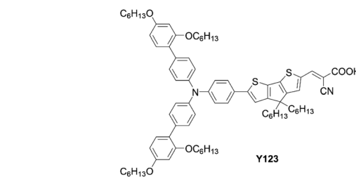
Fig. 17 Chemical structure of Y123 .
