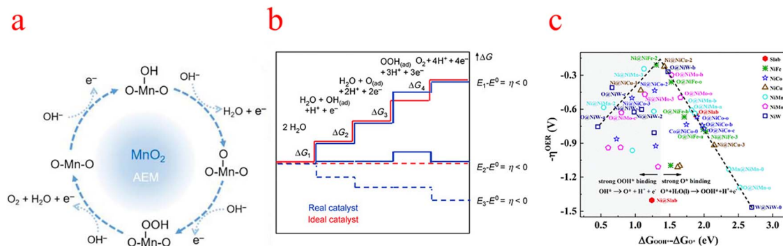
Fig. 1 (a) Schematic diagram of the OER mechanism indicated (using MnO 2 as an example). (b) Gibbs free energy and reaction coordinate diagram of active intermediates (horizontal line) of the OER. The blue line and red line represent the real (typical) catalyst and the ideal catalyst respectively. (c) Overpotential ( -\eta^{\text{OER}} ) Gibbs free binding energy difference with different reaction sites OOH* and O*. (a) Reproduced with permission from ref. 17. Copyright 2023, American Chemical Society. (b) Reproduced with permission from ref. 25. Copyright 2010, John Wiley and Sons. (c) Reproduced with permission from ref. 30. Copyright 2019, Royal Society of Chemistry.
