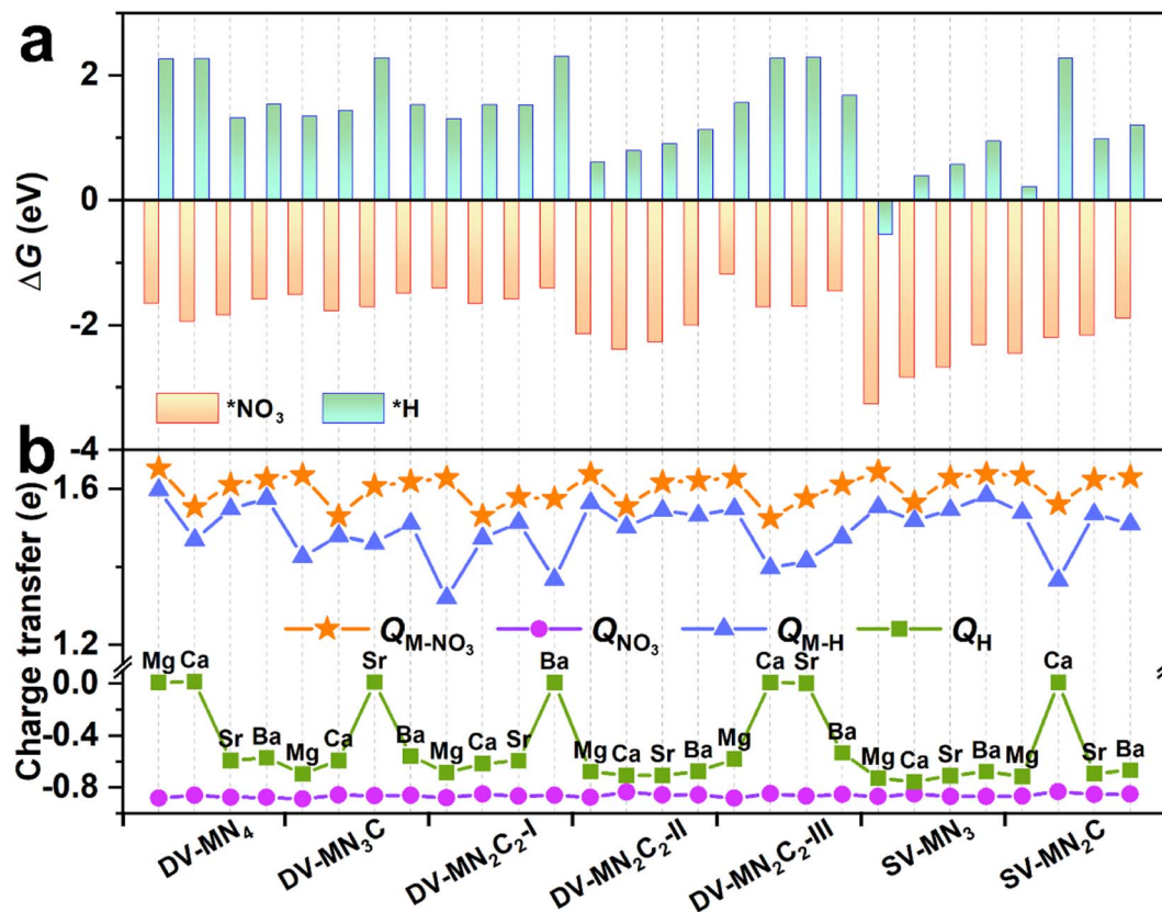
Fig. 3 Adsorption free energy ( \Delta G ) (a) and charge transfer ( Q ) (b) for \text{NO}_3^- and H adsorption on the considered AE-SAC systems. Q_{\text{M-NO}_3^-} and Q_{\text{M-H}} denote the charge transfer of AE metals, and Q_{\text{NO}_3^-} and Q_{\text{H}} are the charge transfer of ^*\text{NO}_3^- and ^*\text{H} , respectively. The positive and negative values represent the electron loss and electron gain, respectively.
