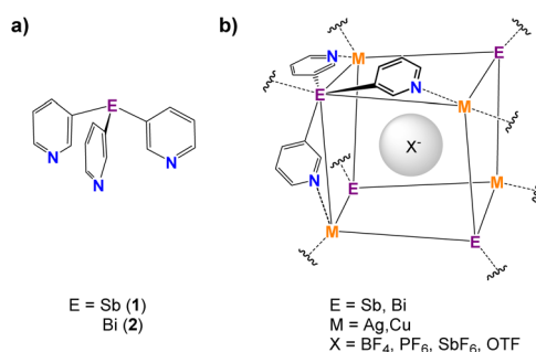
Fig. 2 (a) Antimony- and bismuth-based tris(3-pyridyl) ligands. (b) The \text{E}_4\text{M}_4 unit in the MOFs formed by coordination of 1 and 2 with \text{Cu}^+ and \text{Ag}^+ salts.
