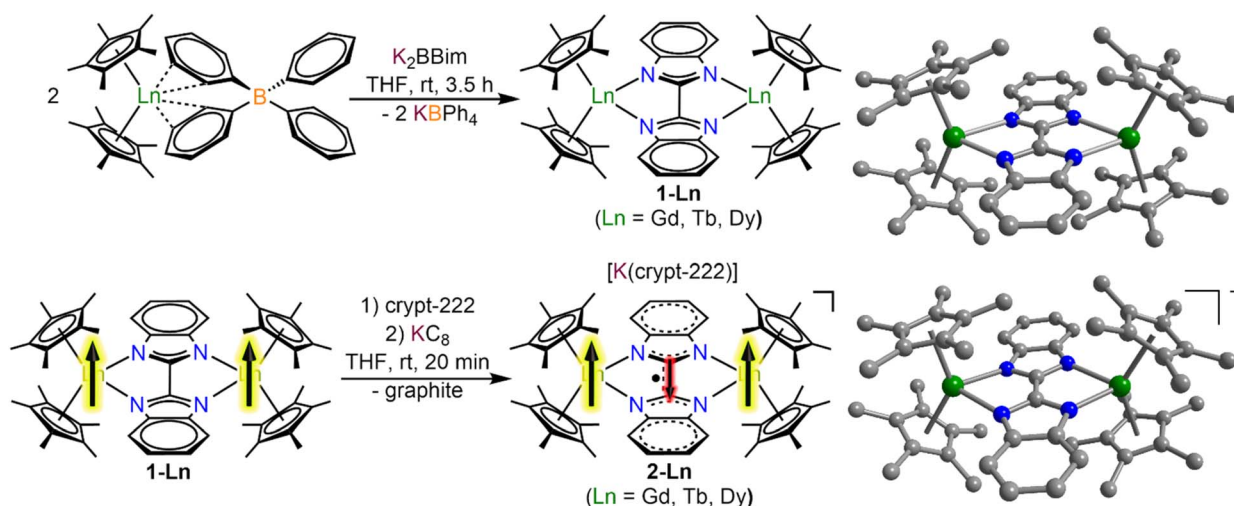
Fig. 1 Synthesis of [(Cp * 2 Ln) 2 (μ-Bbim)] ( 1-Ln ) through salt metathesis reaction of Cp * 2 Ln(BPh 4 ) with K 2 Bbim followed by a reduction of 1-Ln with KC 8 to [K(crypt-222)][(Cp * 2 Ln) 2 (μ-Bbim •− )] ( 2-Ln ). Structures of the Bbim 2- bridged complexes 1-Ln (top) and the Bbim 3•− radical-bridged complexes 2-Ln (bottom). Green, blue and gray spheres represent lanthanide, nitrogen and carbon atoms, respectively. All hydrogen atoms, solvent molecules, and the counter ion ([K(crypt-222)] + for 2-Ln ) are omitted for clarity.
