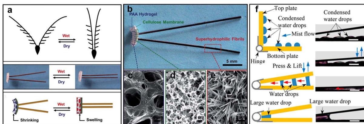
Fig. 15 (a) Schematic diagram of moisture responsive hydrogel driving system in wheat awn shape; (b) the switch consists of three parts: PAA hydrogel, cellulose membrane and super hydrophilic fiber; (c) SEM images of PAA hydrogels prepared by photopolymerization showed porous structure; (d) the SEM images of cellulose films show a porous network structure; (e) the SEM image of \text{Cu}(\text{OH})_2 nanowire coated copper wire shows that the nanowires grow along the copper wire and intersect with each other. 114 This figure has been adapted from ref. 114 with permission from Royal Society of Chemistry, 2015. (f) The fog collection process of a biomimetic fog collector. 115 This figure has been adapted from ref. 115 with permission from American Chemical Society, 2014.
