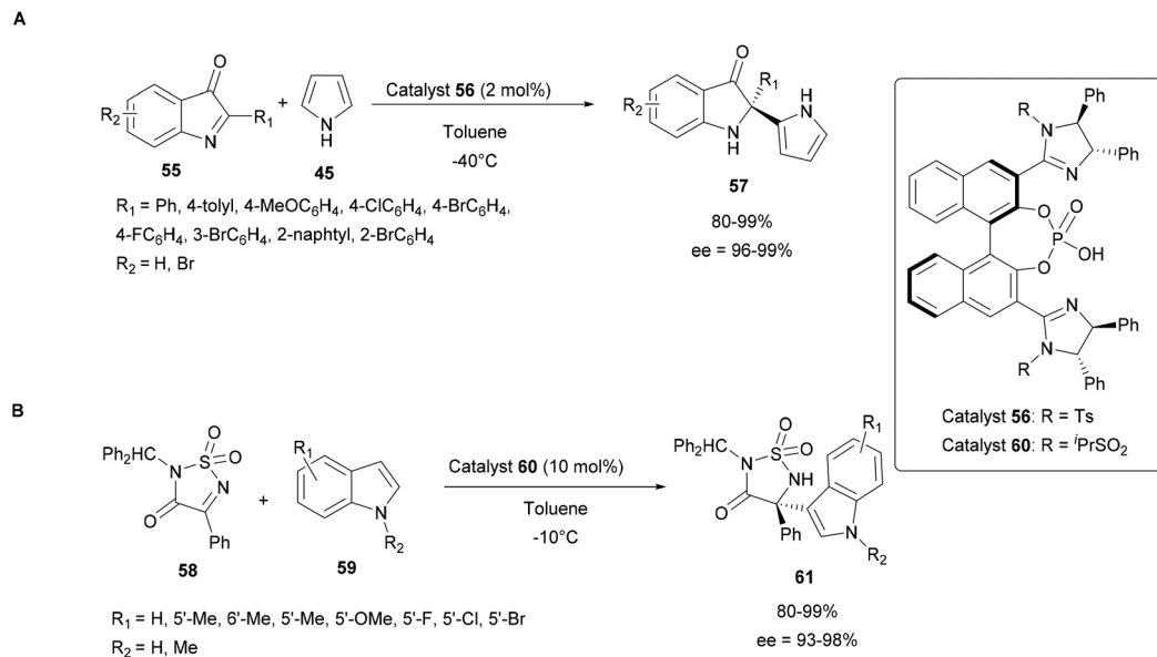
Scheme 16 Organocatalytic enantioselective aza-FC reactions using imidazoline/pyrroles and 3 H -indol-3-ones (A) or cyclic ketimines (B).
