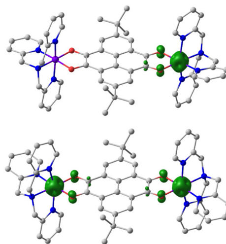
Fig. 9 Spatial structure and spin density distribution (contour value = 0.03 \text{e Å}^{-3} ) of compound 3 in the \{\text{Co}^{\text{III-LS}}(\text{tpa})\text{-pyrene}^{\text{Cat-Sq-CO}^{\text{II-HS}}(\text{tpa})}\} (top) and \{\text{Co}^{\text{II-HS}}(\text{tpa})\text{-pyrene}^{\text{Sq-Sq-CO}^{\text{II-HS}}(\text{tpa})}\} (bottom) charge distributions, as calculated by the DFT UTPSSH/6-311++G(d,p) method. Hydrogen atoms and counter-ions are omitted for clarity.
