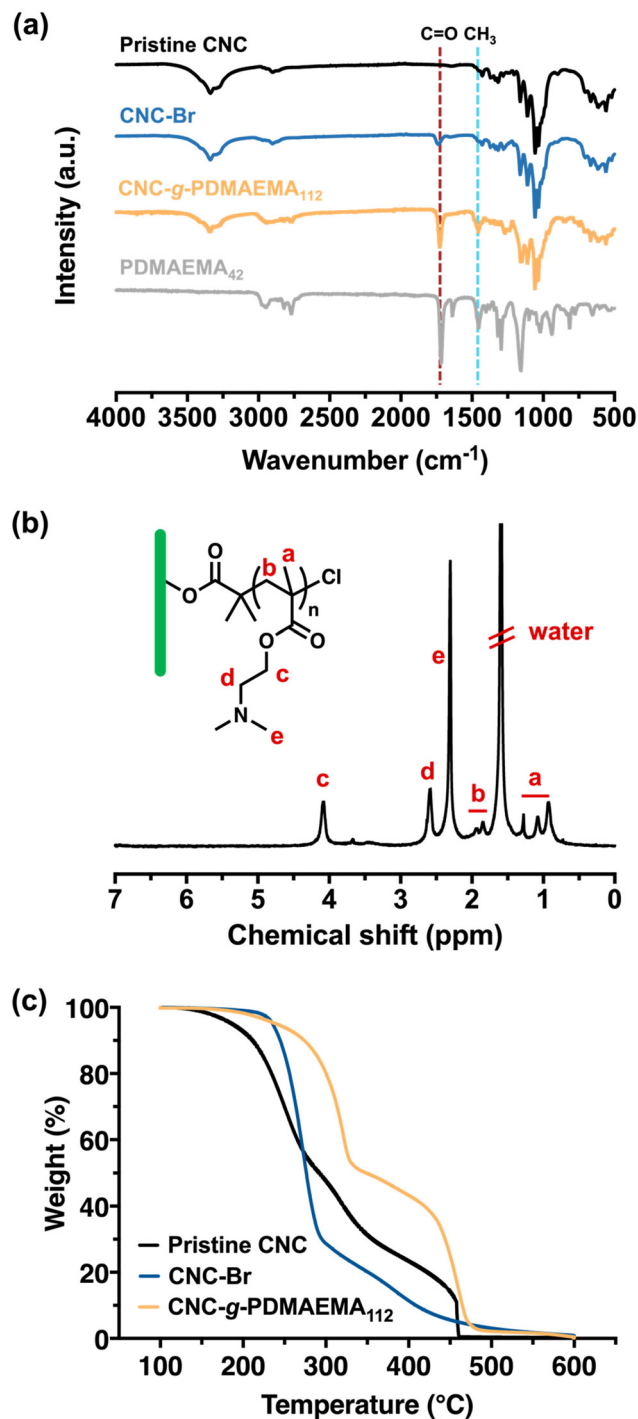
Fig. 1 (a) FTIR spectra of pristine CNC (black), CNC-Br (blue) and CNC-g-PDMAEMA 112 (yellow) and linear PDMAEMA 42 reference (grey). The appearance of a carbonyl peak at 1748 \text{cm}^{-1} confirmed the introduction of ATRP initiator on CNC-Br. The intensifying peaks at 1748 \text{cm}^{-1} and 1442 \text{cm}^{-1} highlighted the presence of the PDMAEMA sidechains. (b) 1 H NMR spectral assignment of CNC-g-PDMAEMA 112 , measured in CDCl 3 . (c) TGA data of the thermal degradation of pristine CNC (black), CNC-Br (blue) and CNC-g-PDMAEMA 112 (yellow) in air.
