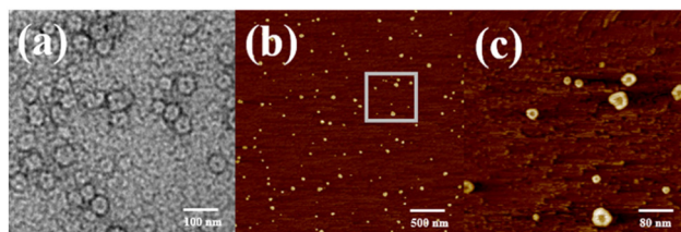
Fig. 6 (a) Negative-staining TEM images and (b) AFM images of cis - \mathbf{H}_1 ( \mathbf{H}_1 after irradiation with 365 nm UV light for 20 min) obtained from 3.03 \times 10^{-6} \text{ mol L}^{-1} \text{H}_2\text{O}/\text{DMSO} ( v/v = 19:1 ) solutions. (c) Enlarged image of part b.
