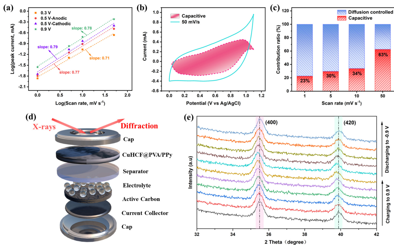
Fig. 5 (a) Determination of b -values for various selected regions for CuHCF@PVA/PPy. (b) Capacitive contribution of CuHCF@PVA/PPy at a scan rate of 50 \text{ mV s}^{-1} . (c) Diffusion-limited and capacitive contributions to the total capacity of CuHCF@PVA/PPy at different scan rates. (d) Schematics of the customised XRD cell for in situ measurements. (e) In situ XRD patterns of the CuHCF@PVA/PPy cell during the desalination/regeneration process at a specific current of 20 \text{ mA g}^{-1} .
