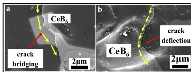
Fig. 16 Crack propagating on the surface of pressureless sintered B_4C -15 wt% SiC ceramics with the sintering aid of 5 wt% CeO_2 : (a) crack bridging and (b) crack deflection 129 (reproduced with permission, Copyright 2013, Elsevier).
