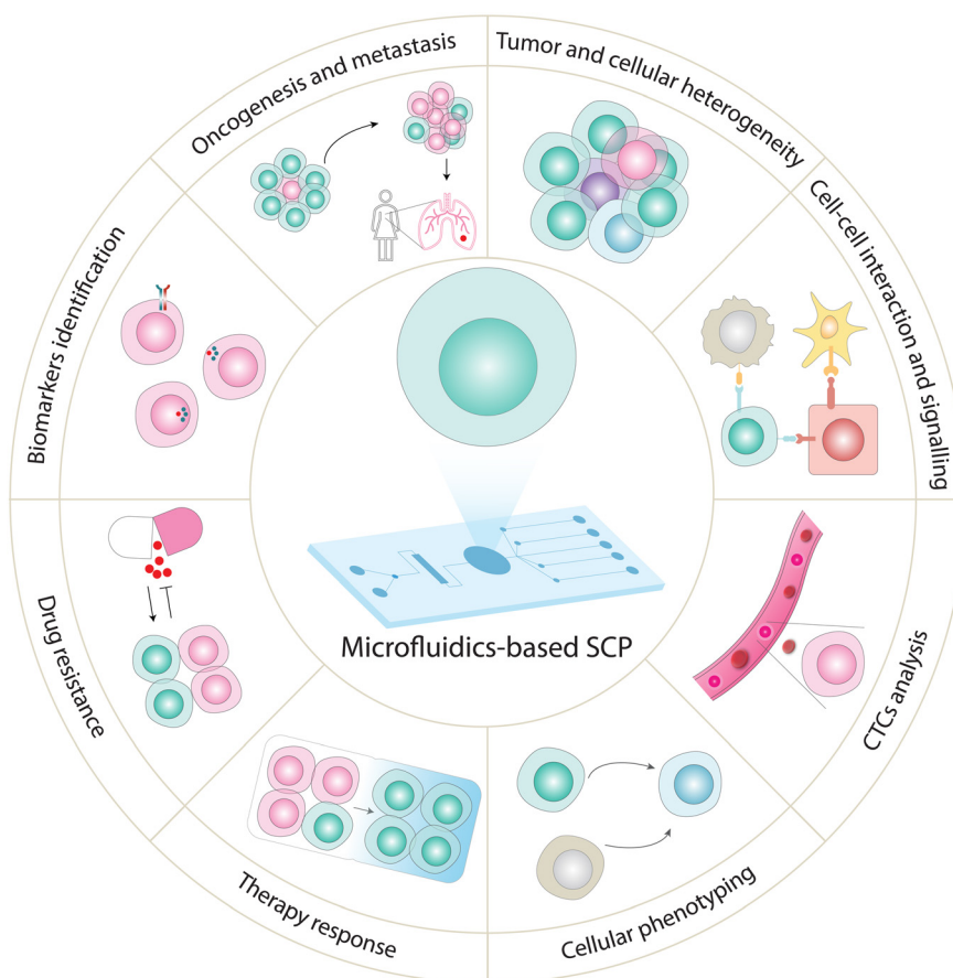
Fig. 5 Emerging applications of SCP analysis using targeted and global approaches. SCP analysis has the potential to measure heterogeneity in different cell lines and dissect tissue heterogeneity, 7,180,231,235,237 explore cancer development and progression, 177 identify biomarkers, 10,238 unveil cellular responses to drugs, 227 investigate mechanistic insights into drug resistance, 108,205,214 profile CTCs (non-invasive diagnosis and real-time cancer monitoring), 231 discover functional proteins to track cellular phenotypes (cell types and cell-state), 7,167 and analyze cellular signaling events. 9,10
