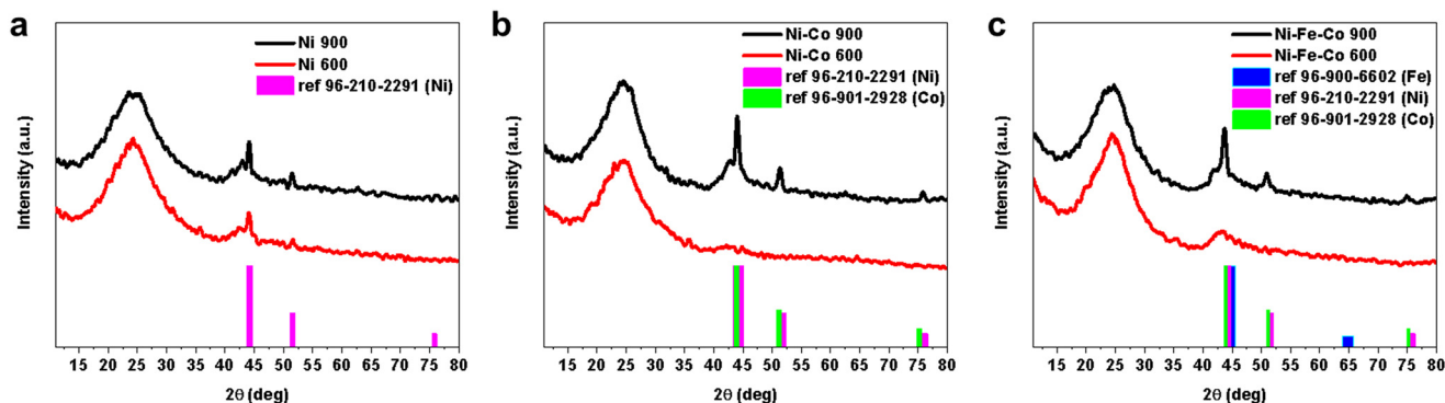
Fig. 5 XRD spectra of Ni-based electrocatalysts with two different functionalization temperatures of 900 °C and 600 °C for the (a) Ni; (b) Ni-Co; and (c) Ni-Fe-Co samples.
