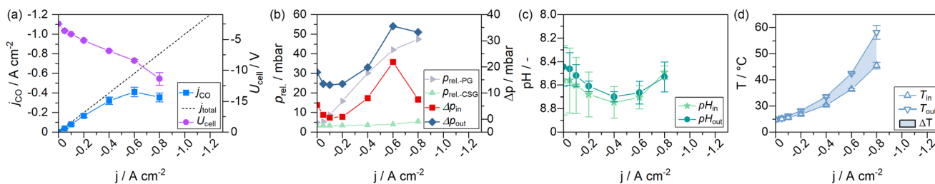
Fig. 4 Current-dependent steady-states of a GDE flow cell operated with 1 M electrolytes. (a) Voltage and CO-specific current density, (b) relative system pressures (PG – product gas, CSG – catholyte sweep gas), (c) and the catholyte pH entering and exiting the GDE flow cell, and (d) the catholyte temperatures entering and exiting the flow cell.
