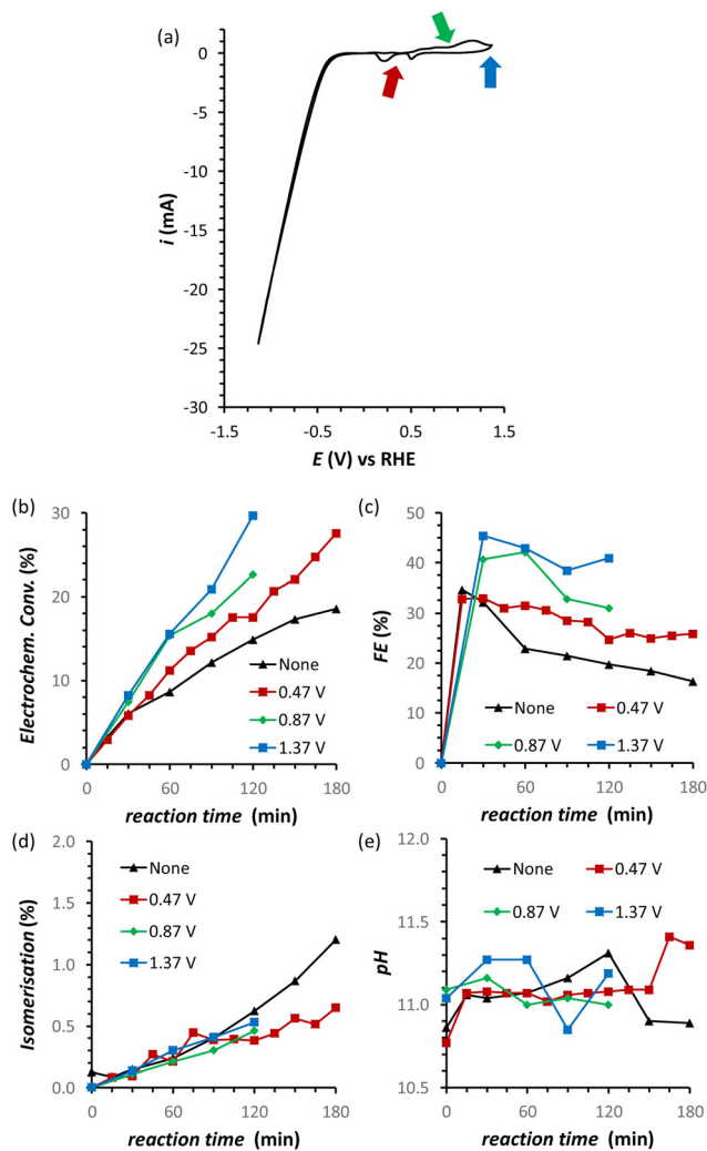
Fig. 6 (a) Cyclic Voltammery (CV) of the Cu-wire electrode at 50 \text{ mV s}^{-1} scan rate sweeping in a potential window from 1.37 \text{ V} to -1.3 \text{ V} vs. RHE. (b–d) Effect of oxidative pulses on the FRR on a Cu-wire electrode in a 0.12 \text{ M} PBS solution at \text{pH}_{\text{initial}} = 11.3 : (b) electrochemical conversion, (c) Faradaic efficiency, (d) isomerisation and (e) the pH. Conditions: i = -20 \text{ mA} ( j = -5.3 \text{ mA cm}^{-2} ), AMVN membrane as separator, constant pH titration with 10 \mu\text{L min}^{-1} of 0.5 \text{ M H}_3\text{PO}_4 , 3 h at room temperature ( 21 \text{ }^\circ\text{C} ).
