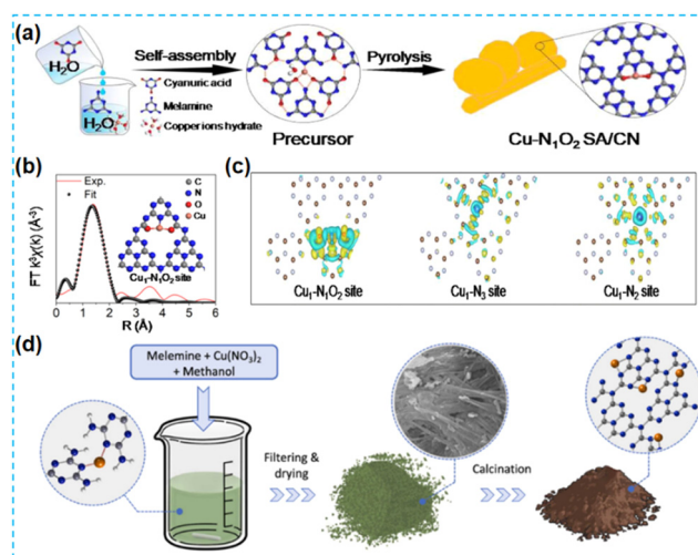
Fig. 22 (a) Schematic illustration of the preparation of SA-Cu-TCN. (b) EXAFS fitting curve in R space and the model of the Cu_1-N_1O_2 site. (c) Differential charge density of Cu_1-N_2 , Cu_1-N_3 , and Cu_1-N_1O_2 coordination configuration. 90 (d) Schematic illustration of the preparation process of CN-xCu samples. 91
