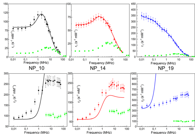
Fig. 2 Longitudinal r_1 (upper) and transverse r_2 (bottom) NMRD profiles of the MNPs in ref. 54 collected at room temperature in the frequency range 0.01 < \nu < 60 MHz and the best-fit curves obtained by applying Roch's model (solid lines). r_1 and r_2 profiles of the (dismissed) commercial compound Endorem® are reported as green symbols in all graphs. 62 Reprinted with permission from ref. [“Tailoring the magnetic core of organic-coated iron oxides nanoparticles to influence their contrast efficiency for magnetic resonance imaging”, M. Basini, A. Guerrini, M. Cobiainchi, F. Orsini, D. Bettega, M. Avolio, C. Innocenti, C. Sangregorio, A. Lascialfari and P. Arosio, J. Alloys Compd. , 2019, 770, 58, doi: https://doi.org/10.1016/j.jallcom.2018.08.120 ]. Copyright 2019, Elsevier.
