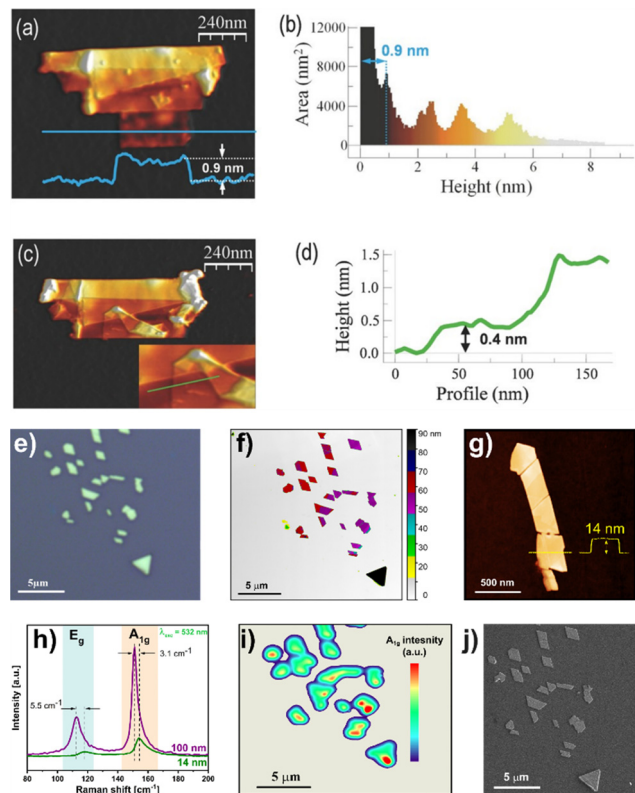
Fig. 10 AFM topography images of an antimonene flake with a monolayer terrace at the bottom. (a) AFM topography showing an antimonene flake with terraces of different heights. (b) Height histogram of the image in (a) pointing out the different thicknesses of the terraces. (c) Same flake as in (a) after a nanomanipulation process to confirm the stability of the material. The lower terrace of the flake was folded upward resulting in an origami structure with different folds. The inset corresponds to the area of the origami where the lowest step height is found. (d) Profile along the green line in the inset in (c). (e) Optical micrograph of a typical antimonene nanosheet isolated on \text{SiO}_2/\text{Si} substrate using micromechanical exfoliation. (f) False-colored AFM image of the same ANSs with incremental color code to highlight the terraces. Each color indicates a 10 nm step. (g) AFM image of a few-layer antimonene nanosheet and height profile along the dashed yellow line. (h) Comparative Raman spectra of the pristine bulk (100 nm) and few-layer (14 nm) antimonene nanosheets, remarking the blue shift of the \text{A}_{1\text{g}} and \text{E}_{\text{g}} modes for the few-layer antimonene nanosheets. (i) Scanning Raman microscopy (SRM) map of the intensity of \text{A}_{1\text{g}} mode of the flakes in (e). (j) Scanning electron microscope (SEM) image of the same flakes in (e). Adapted from ref. 84 with permission from John Wiley & Sons, copyright 2016, and ref. 98 with permission from IOP Publishing, copyright 2020.
