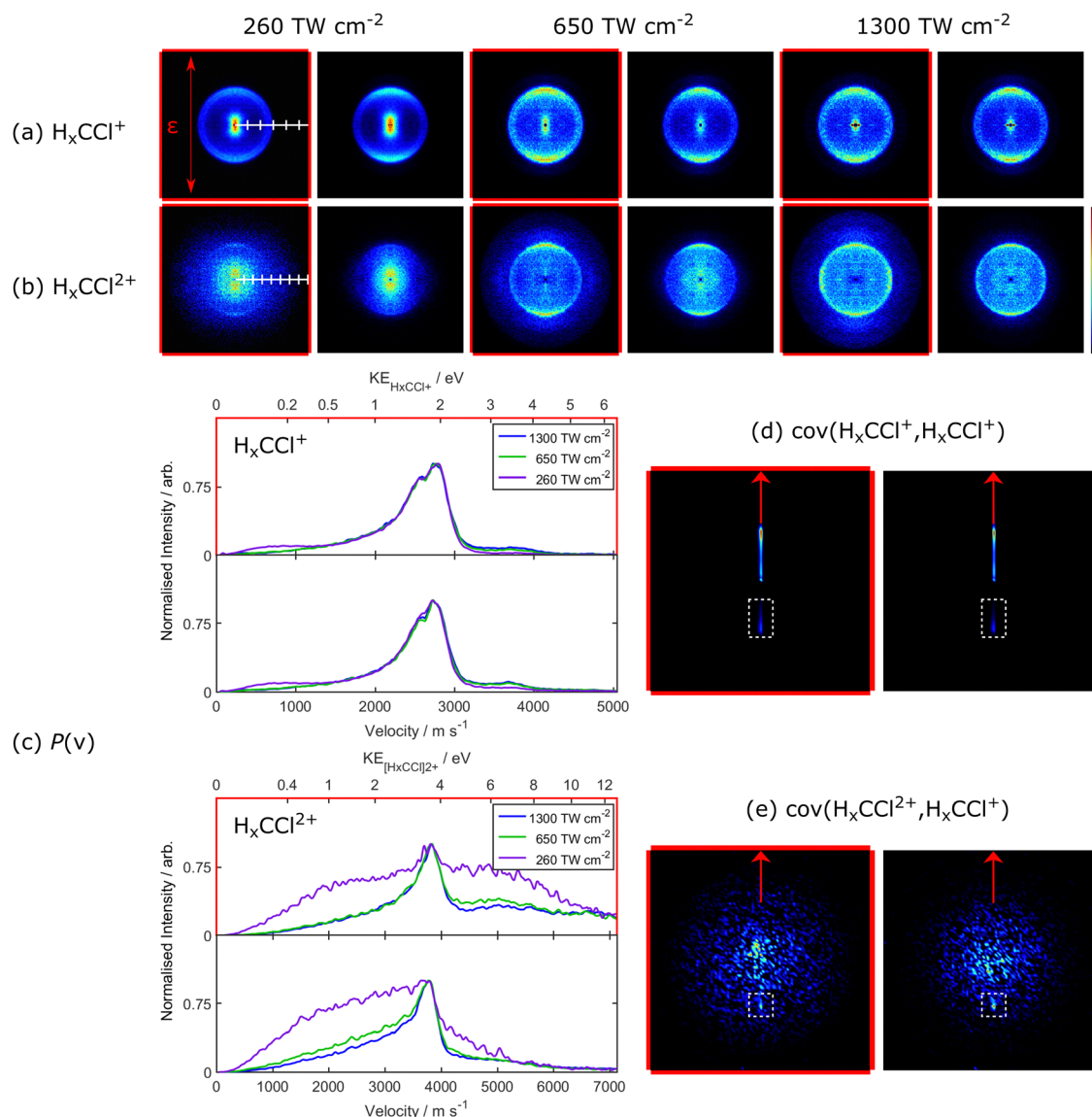
Fig. 6 Symmetrised images of the (a) H_x CCl^+ and (b) H_x CCl^{2+} fragments observed following 805 nm SFI of cis - (red borders) and trans -1,2-DCE at I = 260, 650 and 1300\ TW\ cm^{-2} . The laser polarisation vector, \epsilon , is vertical in the plane of the image, as shown in the top left-hand panel and the relative signal intensities are shown by the linear false-colour scale chosen to span the maximum to minimum signal levels in the regions of interest within each image at the end of row (b). The ticks on the white horizontal scale in the left-hand image in each row indicate 1000 m\ s^{-1} intervals. The P(v) distributions of the H_x CCl^+ and H_x CCl^{2+} fragments from each parent isomer are shown in (c) with, in each case, the maximum signal scaled to an intensity of unity. The corresponding fragment kinetic energies are shown on the top x axis. (d and e) Show, respectively, the (H_x CCl^+, H_x CCl^+) and (H_x CCl^{2+}, H_x CCl^+) covariance map images from analysis of I = 260\ TW\ cm^{-2} data from the cis - (left) and trans -isomers (right), selecting H_x CCl^+ as the reference ion and fixing its velocity to be vertically upwards, as indicated by the red arrow. The covariance signal of interest in each case is bounded by dashed white lines, while the more intense feature along the \phi = 0^\circ axis in both images in (d) is the autovariance signal.
