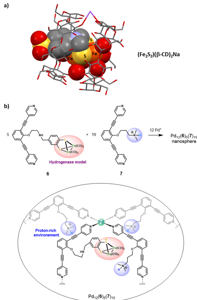
Fig. 7 (a) Representation of the XRD structure of (\text{Fe}_2\text{S}_2)(\beta\text{-CD})_2\text{Na} . (b) Confinement of five hydrogenase mimicking clusters in a proton rich the \text{Pd}_{12}(\text{6})_5(\text{7})_{19} nanosphere (top), along with the schematic representation of one of the five catalytic centers found in the nanosphere (bottom).
