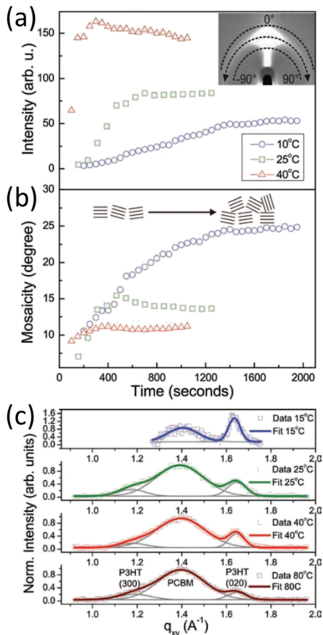
Fig. 24 Evolution of (a) the integrated intensity of the P3HT(100) diffraction peak and (b) mosaicity of P3HT, which was deduced from the (100) peak width, during blade coating of P3HT:PC 61 BM at different substrate temperatures. (c) Ex situ GIWAXS data along the in-plane direction of the dry films coated at different temperatures. Adapted with permission. 99 Copyright 2011, Wiley-VCH Verlag GmbH & Co. KGaA, Weinheim.
