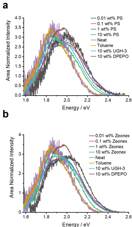
Fig. 4 Prompt fluorescence spectra (0.8 ns after excitation) extracted from the time-resolved emission decays of 4DTPIP in the various solid films and in toluene solution at room temperature.
