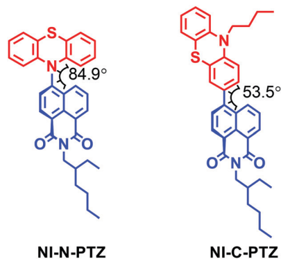
Fig. 6 Molecular structure of NI-N-PTZ , which shows TADF properties. The molecular structure of the reference compound NI-C-PTZ is also presented. Reproduced with permission. 67 Copyright 2019, American Chemical Society.
