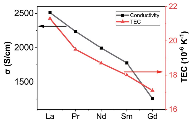
Fig. 3 Variation of DC electrical conductivity ( \sigma ) and thermal expansion coefficient (TEC) in \text{Ln}_{0.6}\text{Sr}_{0.4}\text{CoO}_{3-\delta} ( \text{Ln} = \text{La}, \text{Pr}, \text{Nd}, \text{Sm} and \text{Gd} ) in air. Values are extracted from ref. 70, 76, 81, 90 and 91.
