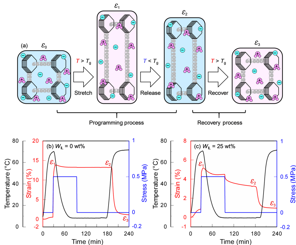
Fig. 3 (a) Schematic diagram of the shape memory effect of an ionic SMP gel. TMA curves of (b) SMPs ( W_{\text{IL}} = 0 wt%) and (c) ionic SMP gels ( W_{\text{IL}} = 25 wt%) where temperature (on the left of the plot), strain, and stress curves correspond to black, red, and blue lines, respectively. The specimen (5 mm long, 2 mm wide, and ca. 300 \mu\text{m} thick) was first heated to 70 ^{\circ}\text{C} above T_g at a heating rate of 5 ^{\circ}\text{C min}^{-1} and stretched under a constant stress of 0.5 MPa, then cooled down to ca. 10 ^{\circ}\text{C} to fix the shape with a temporary strain of \varepsilon_1 . After releasing the stress, the sample slightly relaxed with a fixed strain of \varepsilon_2 . Finally, the sample recovered from its temporary shape to the original shape with a recovery strain of \varepsilon_3 by heating again from room temperature to 70 ^{\circ}\text{C} .
