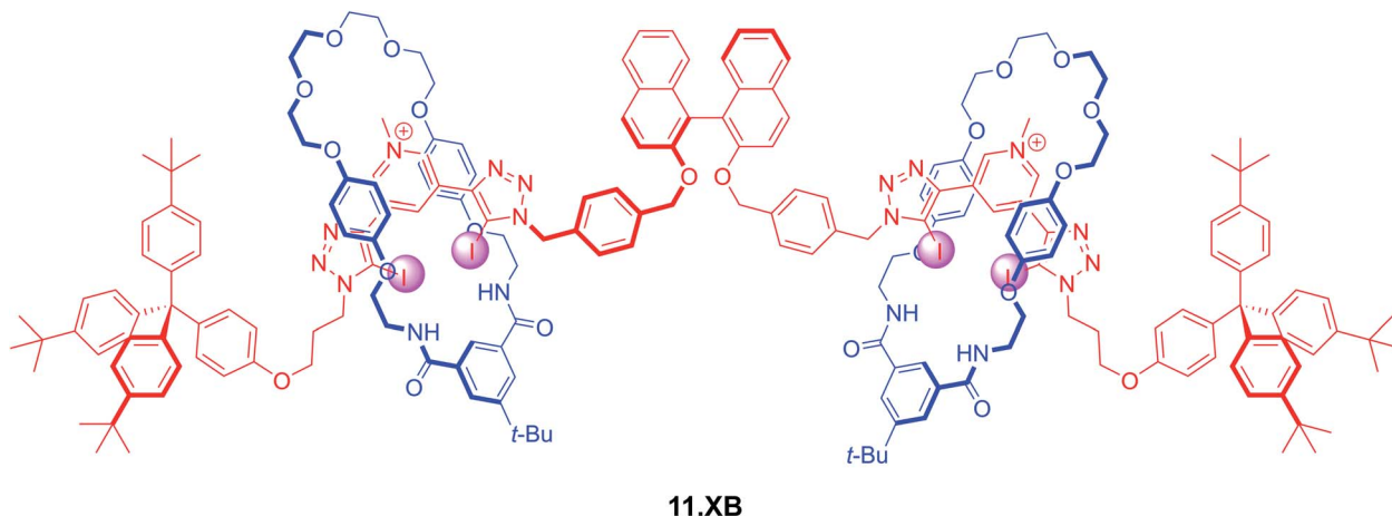
Fig. 14 S -BINOL-based fluorescent [3]rotaxane 11.XB for fluorescent discrimination of S / R -glutamate enantiomers and fumarate/maleate geometric dicarboxylate isomers in CHCl 3 /MeOH/H 2 O 60 : 39 : 1.
