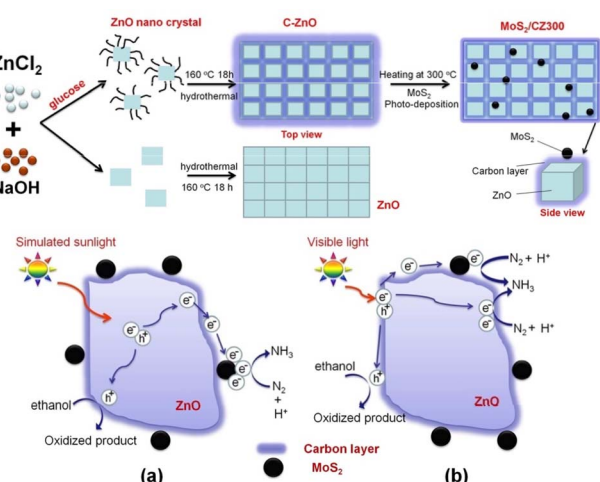
Fig. 11 Preparation of MoS 2 /CZ300 photocatalyst and the suggested charge transfer mechanism of MoS 2 /CZ300 composite (a) under simulated sunlight (b) and visible light irradiation. Reproduced from ref. 79 with permission from [American Chemical Society], copyright [2018].
