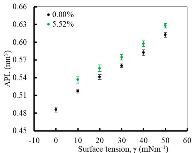
Fig. 2 The APL values of the lung surfactant monolayer as a function of surface tension in the absence and presence of 5.52% w/w of glucocorticoid drug hydrocortisone for the surfactant protein containing monolayer. The error bars indicate standard deviation of the time evolution of APL data across the frames of the trajectories.
