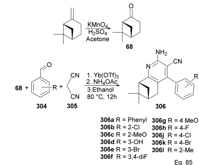
Scheme 79 Synthesis of 2-amino-3-cyanopyridines from (+)-nopinone.
