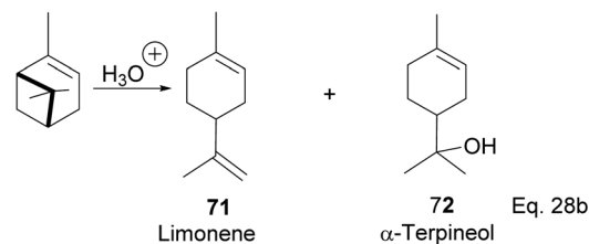
Scheme 24 Acid-catalyzed hydration of \alpha -pinene to monocyclic terpenoid derivatives.
