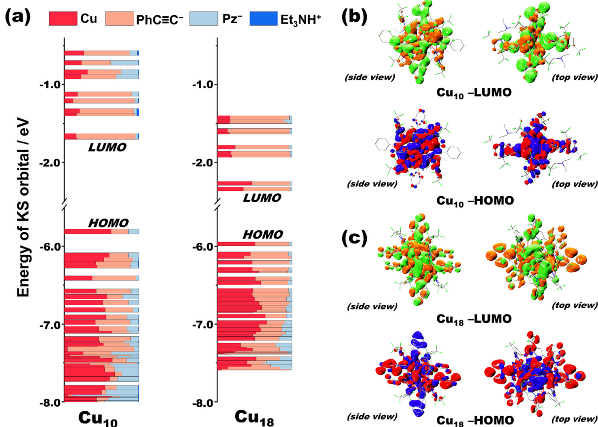
Fig. 5 Composition analysis of Kohn–Sham orbitals of \text{Cu}_{10} and \text{Cu}_{18} . (a) Electronic density diagrams of the HOMO and LUMO of (b) \text{Cu}_{10} and (c) \text{Cu}_{18} (side view and top view). H atoms are omitted for clarity.
