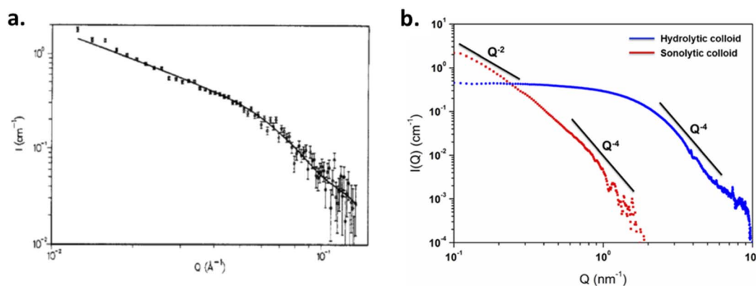
Fig. 10 (a) SANS diagram acquired on Pu colloids prepared in aqueous solution (total Pu 0.12 M) which measured 4.7 nm × 190 nm according to data simulations. Adapted from ref. 100 with permission from the American Chemical Society, copyright 1990. (b) SAXS diagrams acquired for 10 mM hydrolytic and 0.8 mM sonolytic colloids. Black lines indicate the slope power laws. The slope observed for the hydrolytic colloid is typical for 3D objects and compact particles (2.6 nm according to simulations). The one observed for the sonolytic colloid is characteristic of elongated objects (e.g. thin disks or lamellas measuring 5.7 nm × > 30 nm according to simulations). Reproduced from ref. 94 with permission from the Royal Society of Chemistry, copyright 2020.
