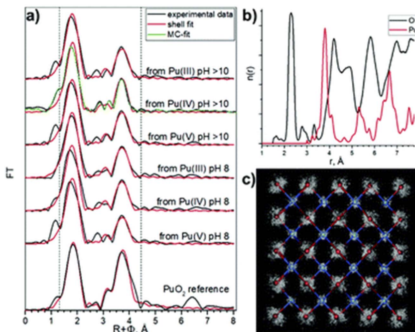
Fig. 14 (a) FT magnitude of experimental Pu L_3 EXAFS spectra (black) acquired on \text{PuO}_2 nanoparticles prepared by ammonia addition into \text{Pu(III)} – \text{Pu(V)} aqueous solutions. \chi(R) fit results obtained with one Pu–O and one Pu–Pu shell fit are represented in red and Monte-Carlo simulation fits are represented in green. The two vertical dashed lines represent the area of the shell fit. (b) Radial particle distribution function ( n(r) ) for Pu–O and Pu–Pu obtained for Monte-Carlo simulation and (c) 3D structural refinement based on bulk \text{PuO}_2 structure. Reproduced from ref. 111 with permission from the Royal Society of Chemistry, copyright 2020.
