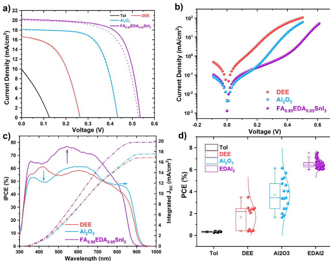
Fig. 4 Enabling FASnI 3 solar cells by antisolvent selection and Al 2 O 3 interlayer and EDAl 2 improves reproducibility and performance. (a) The best J - V curves under simulated AM 1.5 G measured for FASnI 3 -based solar cells with Tol, DEE, Al 2 O 3 and EDAl 2 conditions. Both forward (solid lines) and reverse (dot lines) measurements are indicated. (b) Dark J - V curves for DEE, Al 2 O 3 and EDAl 2 solar cells, showing a substantial reduction in the leakage current (the current density at 0 V). (c) IPCE and Integrated J sc for DEE, Al 2 O 3 and EDAl 2 solar cells. (d) Statistical distribution of PCE for the different devices discussed in this work.
