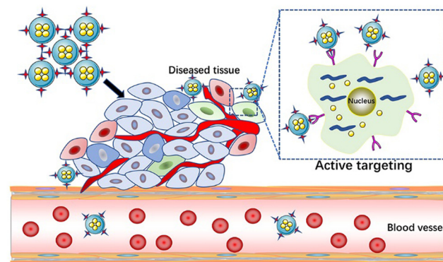
Fig. 2 Schematic diagram of active targeted release.
