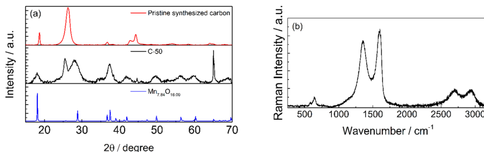
Fig. 4 (a) X-ray diffraction patterns of pristine synthesized carbon (red), C-50 (black) and diffractogram of Mn 7.84 O 16 (reference code 96-151-4117). (b) Raman spectrum of the carbon ground in an agate mortar.
