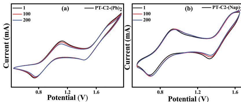
Fig. 4 Cyclic voltammograms ( 200 \text{ mV s}^{-1} ) of PT-C2-(Ph) _2 (a) and PT-C2-(Nap) _2 (b) (1st, 100th and 200th cycles) in DCM (ca. 1.0 mM) recorded in \text{CH}_2\text{Cl}_2 using TBAPF _6 (0.1 M) as the supporting electrolyte.
